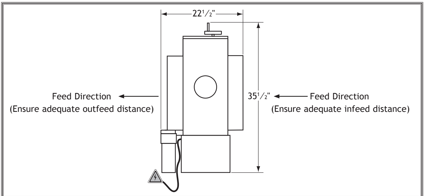
Figure 3. Working clearances.
