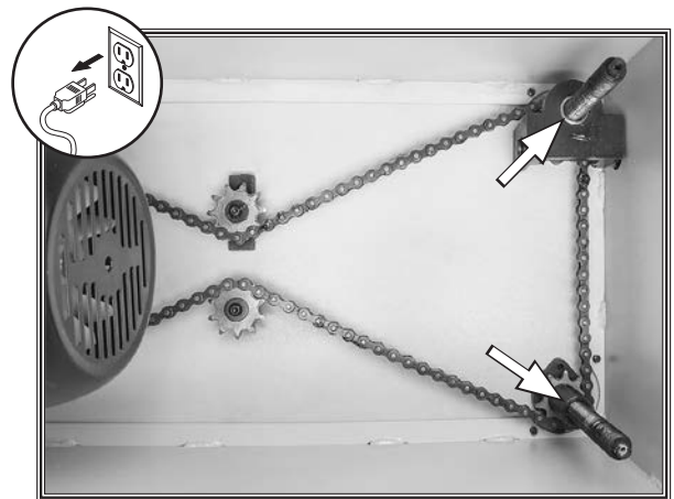
Figure 26. Table lift screws (2 of 4).
