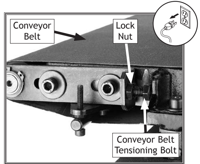
Figure 37. Conveyor belt tensioning controls (outside of table shown).
