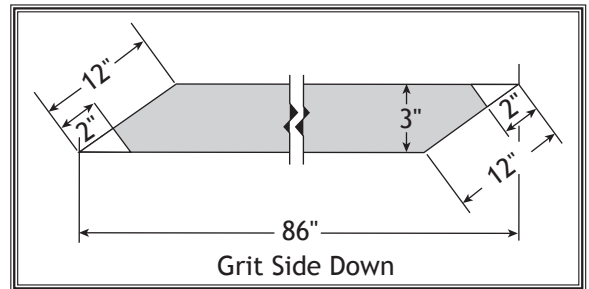
Figure 18. Sandpaper pattern for drum.
