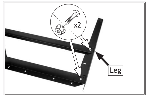
Figure 5. A completed stand leg assembly.
