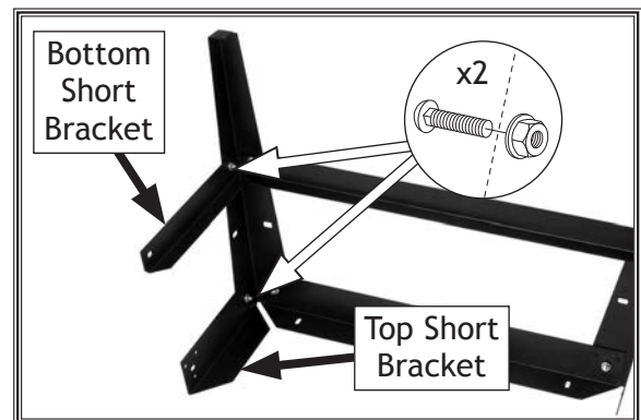
Figure 6. Top and bottom short brackets secured to stand leg assembly.
