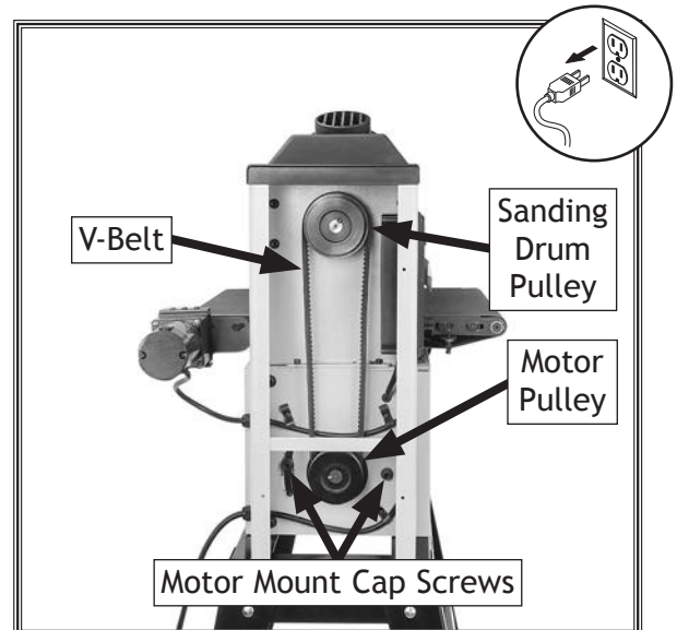
Figure 29. V-belt replacement adjustments.
