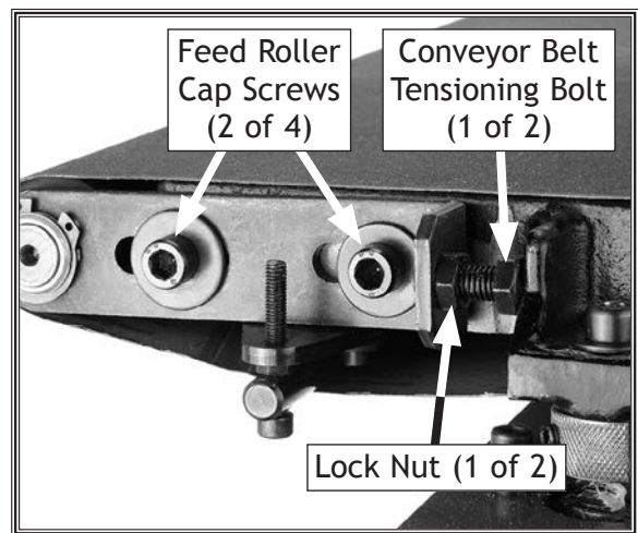
Figure 36. Conveyor belt tensioning controls.
