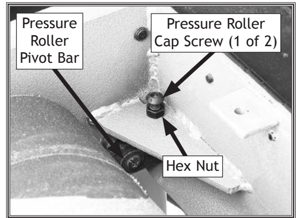
Figure 45. Rear pressure roller adjustments.
