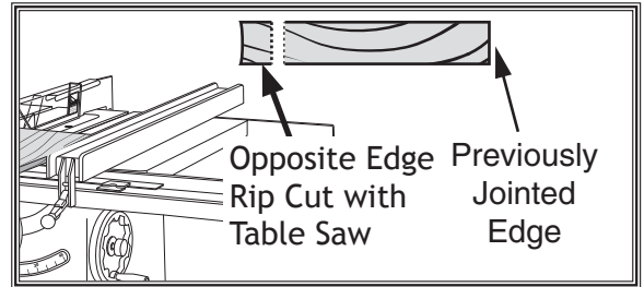
Figure 40. Rip cutting on a table saw.
