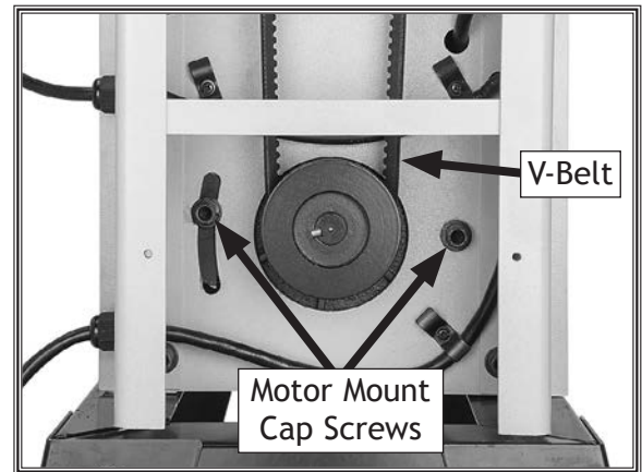
Figure 31. V-belt tension adjustments.
