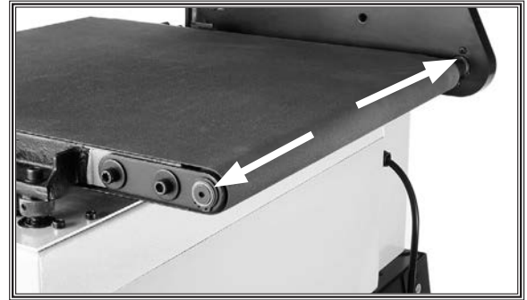
Figure 25. Conveyor belt bushing locations (drive-motor end).
