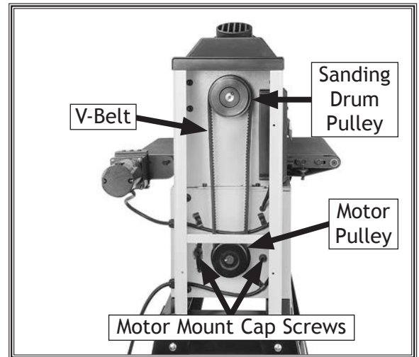
Figure 33. Belt-drive system.
