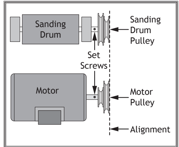
Figure 32. Pulleys must be parallel and aligned.
