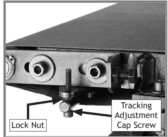
Figure 35. Conveyor fine tracking controls.
