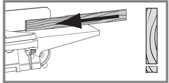
Figure 39. Edge jointing on a jointer.
