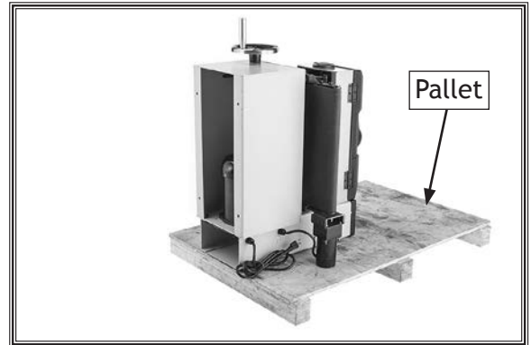
Figure 8. Sander tipped back on pallet against belt access panel.
