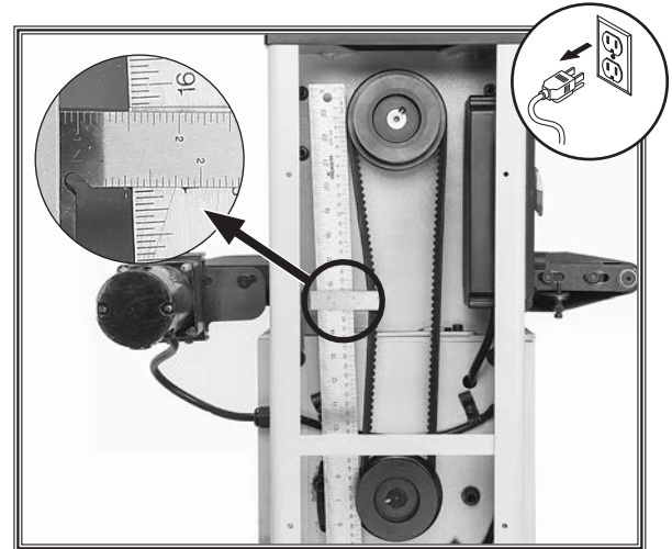
Figure 30. Checking V-belt tension with a straightedge and fine ruler.
