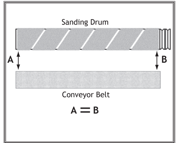
Figure 41. Drum parallel to conveyor belt.
