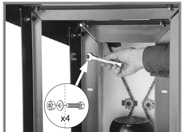
Figure 10. Mounting sander to stand.
