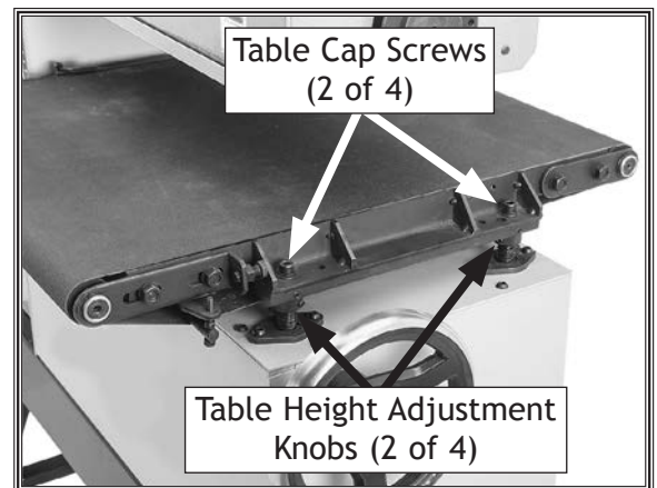
Figure 43. Table height adjustment knobs (outside knobs shown).
