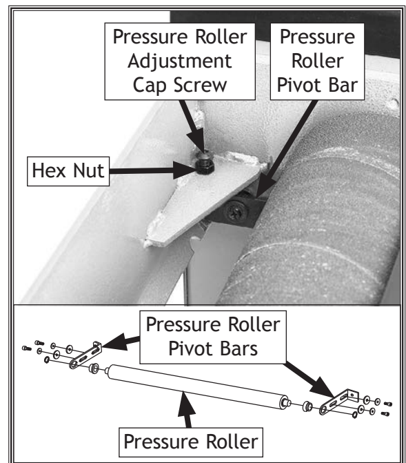
Figure 46. Front pressure roller adjustments and pressure roller overview.
