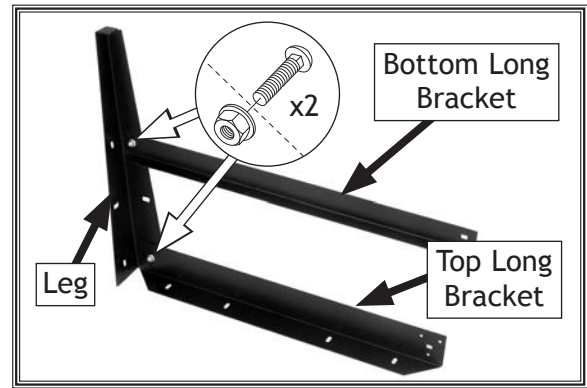
Figure 4. Top and bottom long brackets secured to a stand leg.
