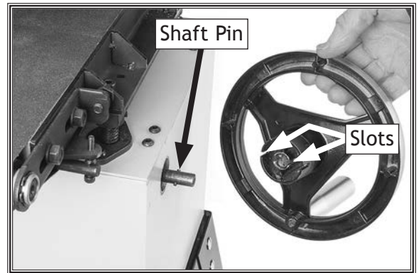
Figure 12. Installing handwheel.
