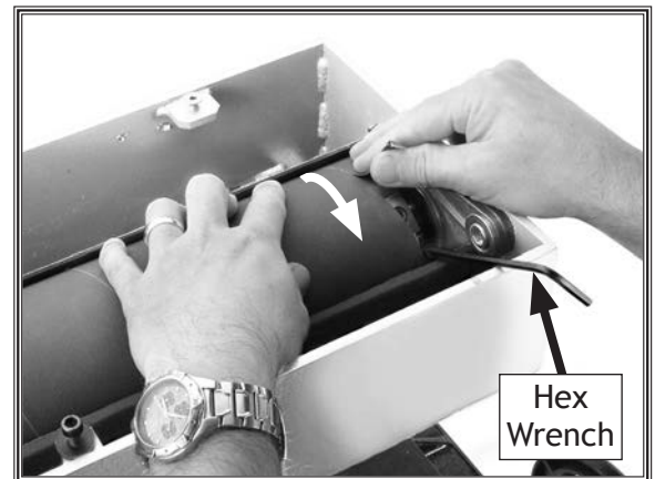
Figure 22. Wrapping sandpaper over tension wheel.
