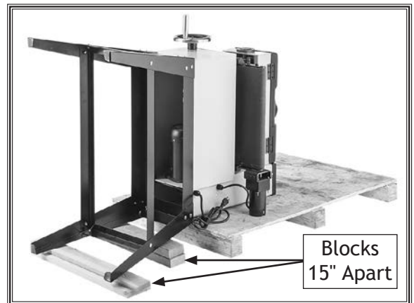
Figure 9. Stand resting on blocks.
