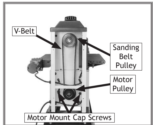
Figure 24. Belt-drive system.
