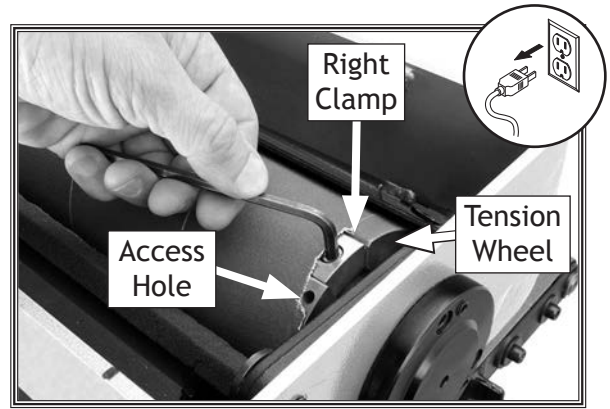
Figure 17. Loosening cap screw on right spring-loaded clamp.
