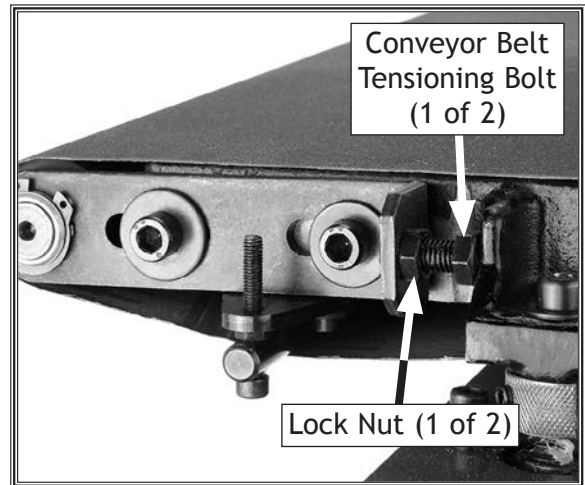
Figure 34. Conveyor coarse tracking controls.
