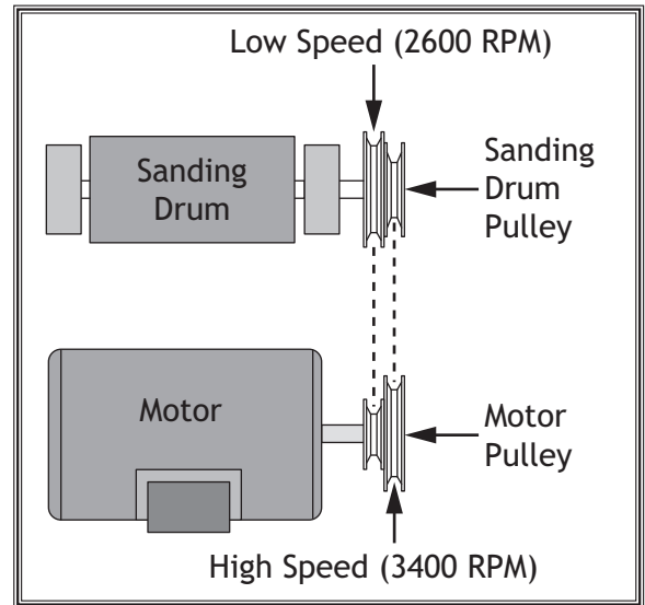
Figure 23. Pulley speed settings.
